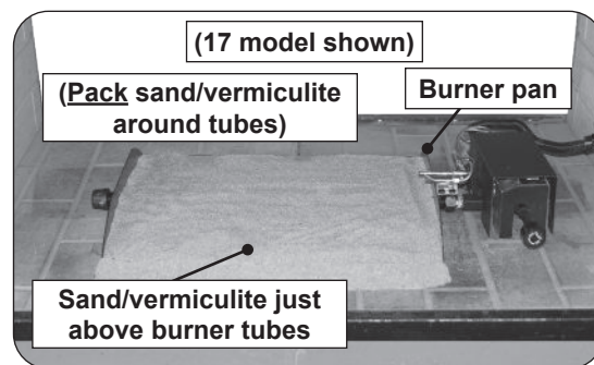
Fig. 19-1 Place sand/vermiculite
