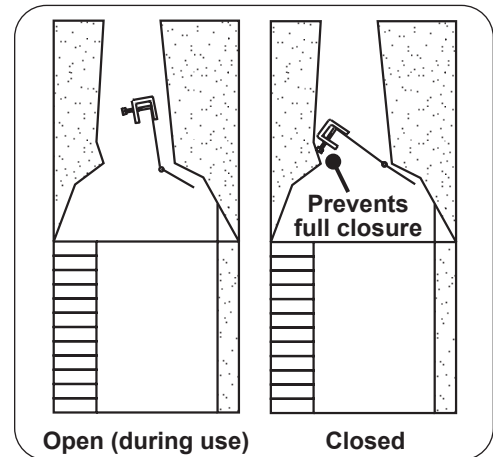
Fig. 9-2 Damper open / closed
