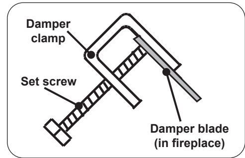
Fig. 9-1 Damper clamp detail
