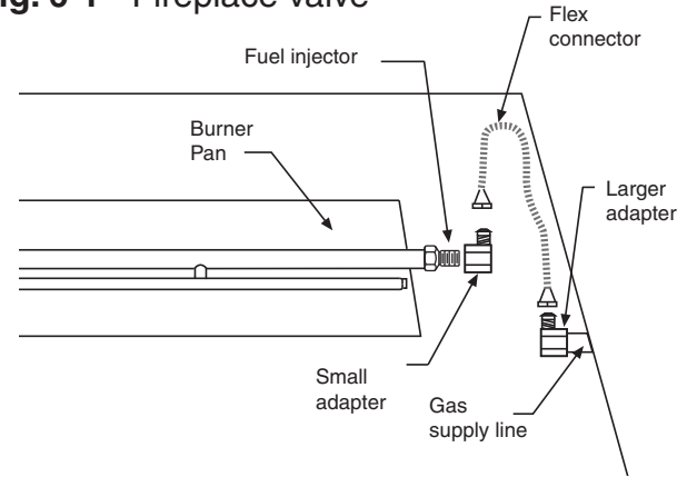
Fig. 6-1 - Fireplace valve
