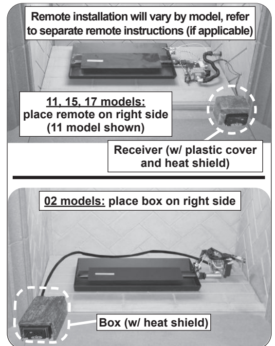
Fig. 17-2 Install remote receiver and heat shield (as applicable)
